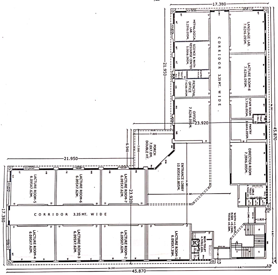
GROUND FLOOR PLAN (BLOCK-C)
